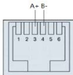
RS485 interface
